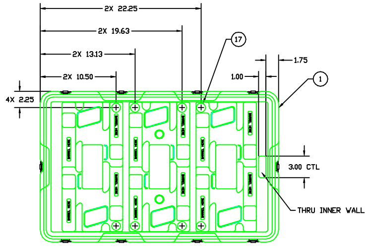
TOP VIEW WITH LID AND TRAY REMOVED
